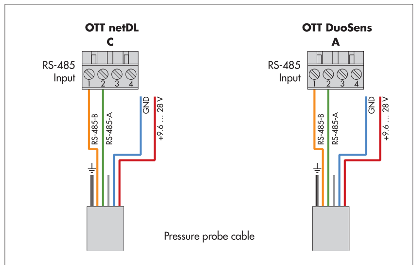
Fig. 10: Connecting the OTT PLS to a to an OTT netDL or OTT DuoSens using an RS-485 interface (SDI-12 protocol).
